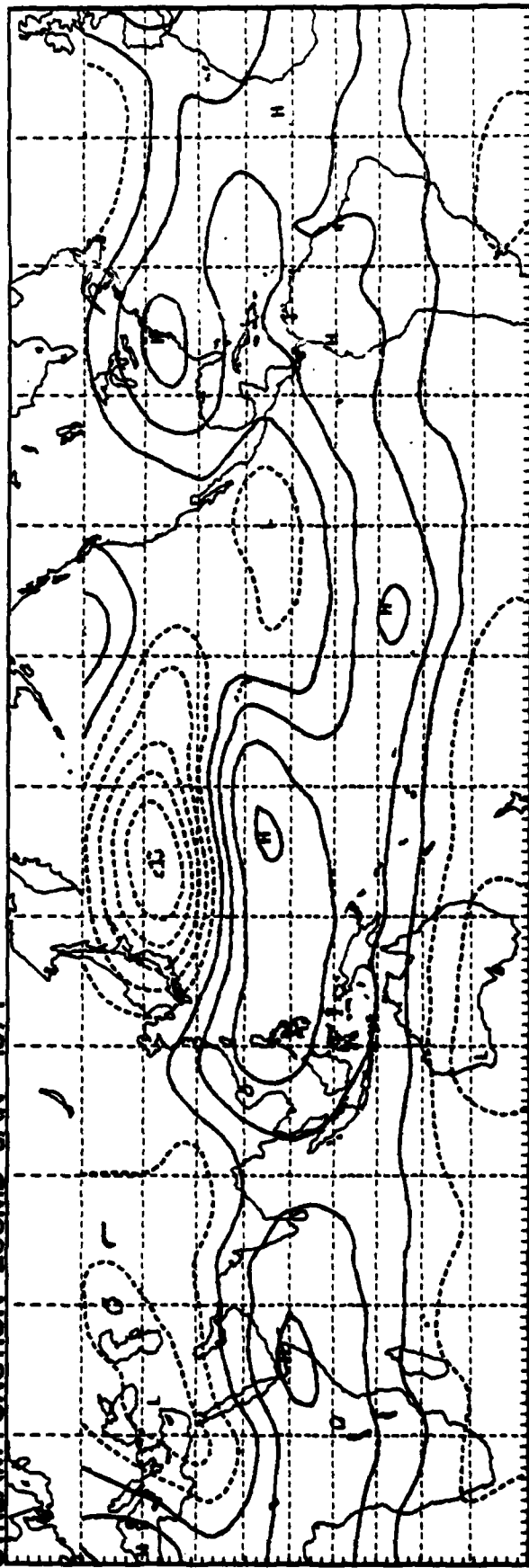
STREAM FUNCTION 200MB JAN 1974
